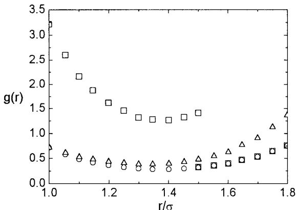
Fig. 1. Monte Carlo simulation results (10) for the structure functions g(r) (squares), y(r) (circles), and \psi(r) (triangles) on a SW fluid with \lambda=3/2 , T^*=2/3 and \eta=2\pi/15 . Note that g(r) and y(r) overlap for r > \lambda\sigma .
