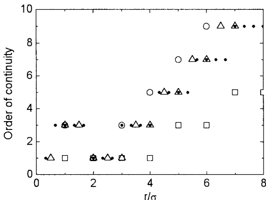
Fig. 2. Order of continuity of y(r) versus r/\sigma for the SW fluid with \lambda=2 (squares), \lambda=3/2 (triangles), and \lambda=4/3 (dots), and the HS fluid (circles). The order of continuity is assumed to be infinity if not plotted.
